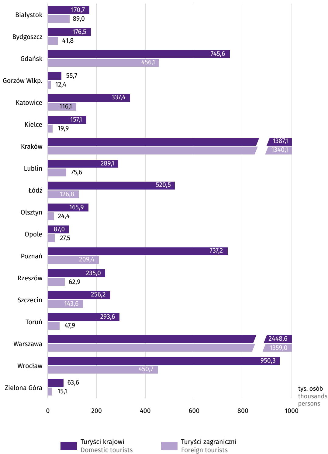
Chart 32. Tourists accommodated in tourist accommodation facilities in January-December 2019
